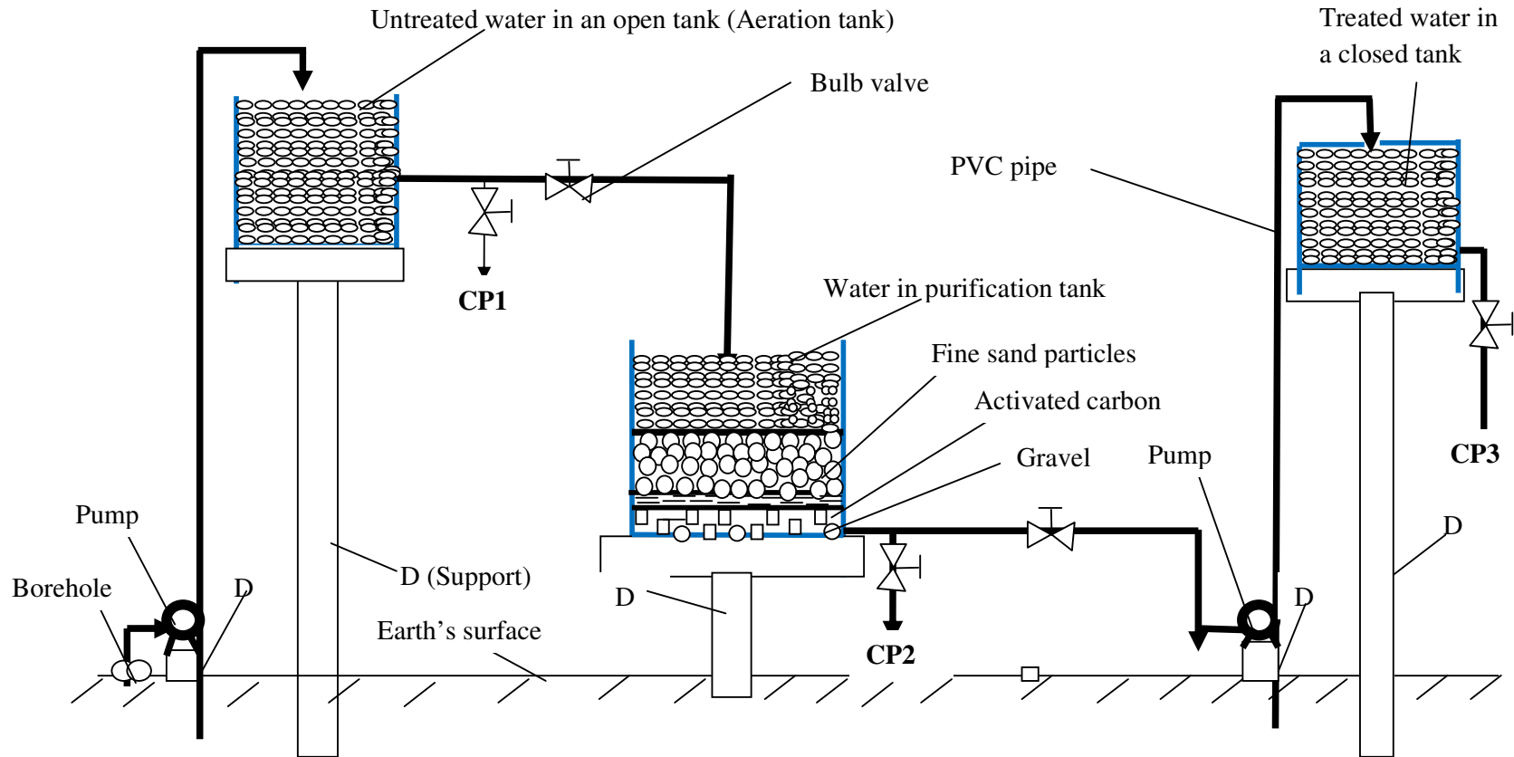
Figure 2: A simplified diagram of a borehole water purification system. CP1, CP2 and CP3 are water collection points. D is a support or stand.
