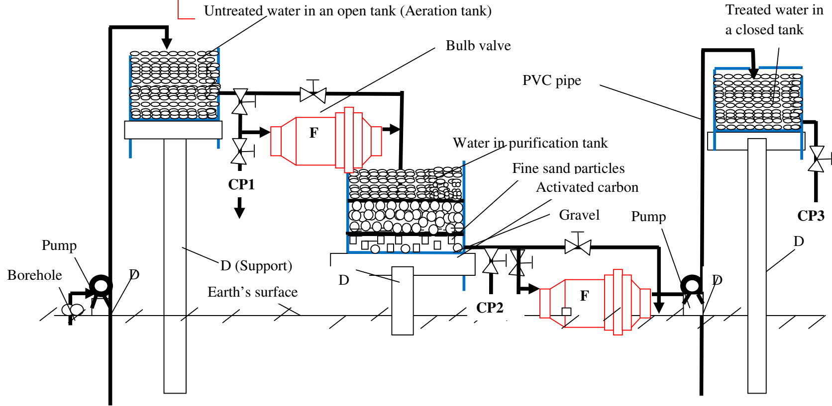
Figure 3: A simplified diagram of a borehole water purification system showing the possible positions of the portable tubular filter pipe (F).
