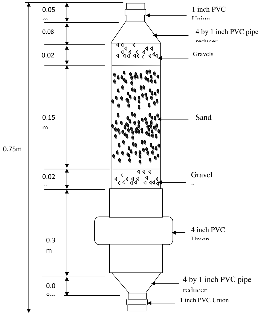
Figure 4: The design drawing of the Portable Tubular Filter Pipe
