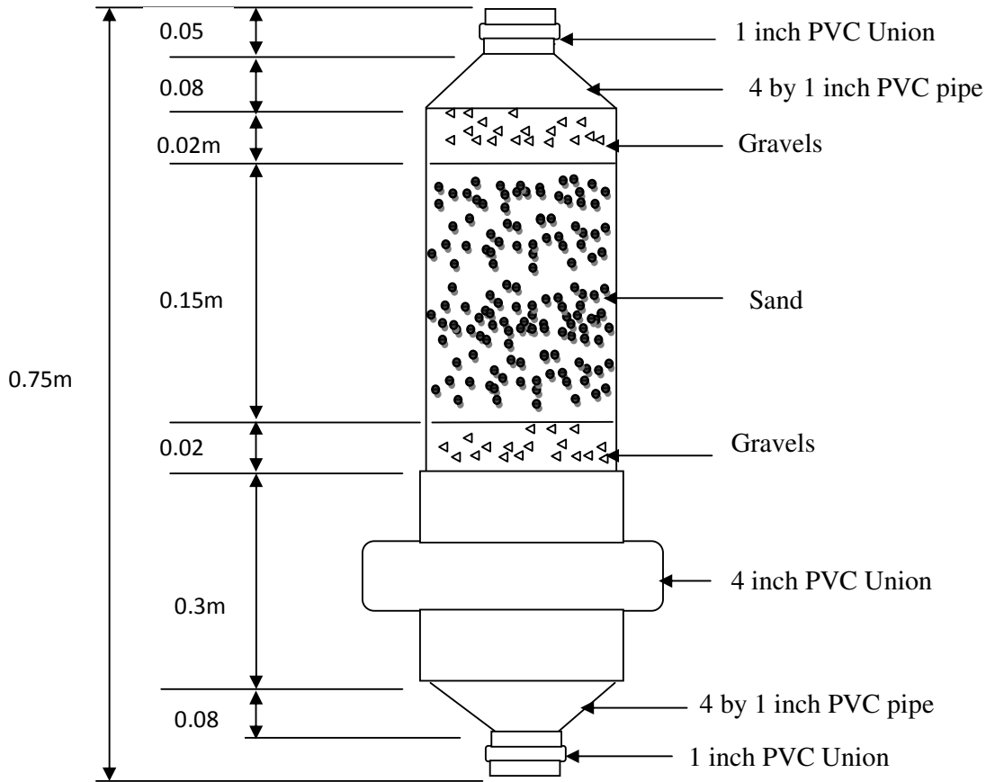
Figure 4: The design drawing of the Portable Tubular Filter Pipe
