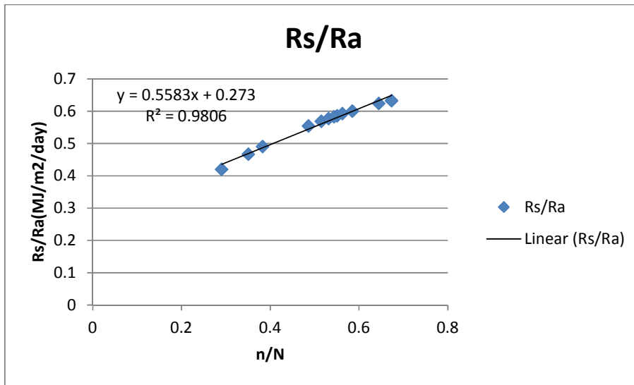
Figure 4: Angstrom-Prescott (1940) model fitting for variation of clearness index ( R_s/R_a ) versus sunshine duration ( n/N ) for Makurdi (1999 - 2008)
