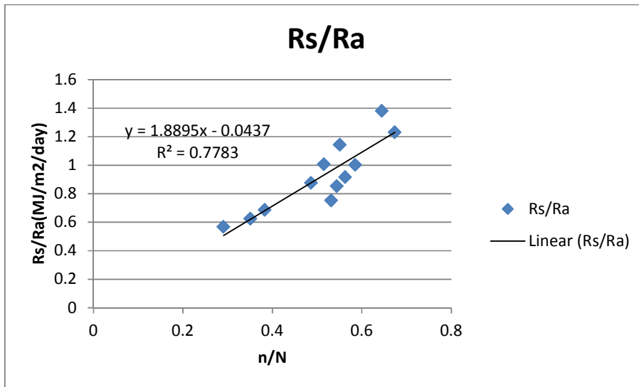
Figure 9: Annadale (2002) model fitting for variation of clearness index ( R_s/R_a ) versus sunshine duration ( n/N ) for Makurdi (1999-2008)
