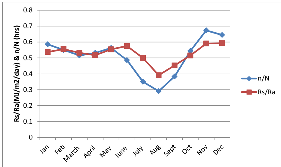
Figure 1: Correlation of monthly variation of R_s/R_a and n/N for Makurdi (1999 - 2008)
