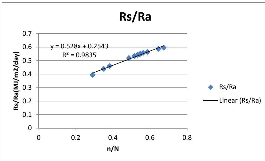
Figure 5: Louche (1991) model fitting for variation of clearness index ( R_s/R_a ) versus sunshine duration ( S/S_o ) for Makurdi (1999 - 2008)
