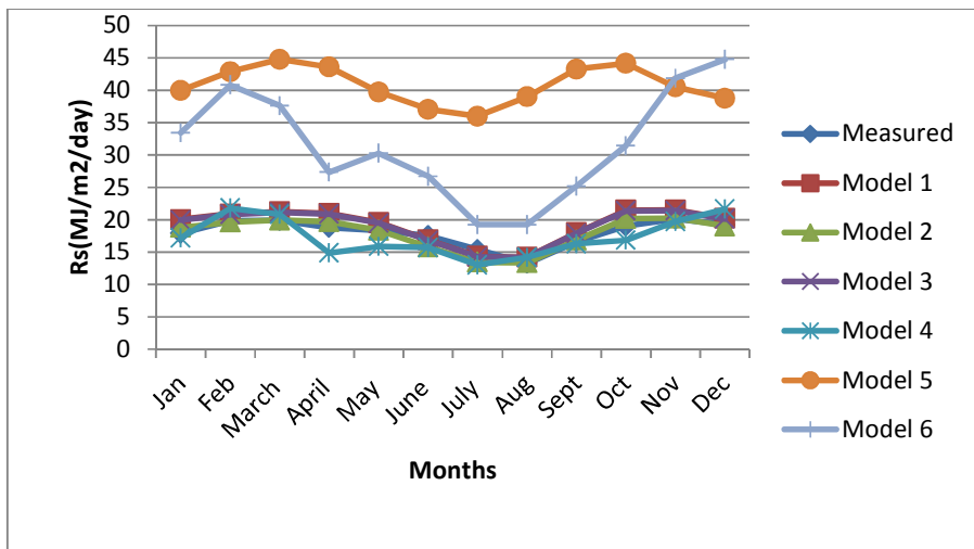
Figure 3: Measured and estimated monthly mean global solar radiation for Makurdi (1999-2008)
