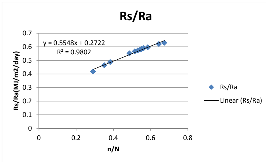
Figure 6: Glover Mc-culloch (1958) model fitting for variation of clearness index ( R_s/R_a ) versus sunshine duration ( n/N ) for Makurdi (1999 - 2008)
