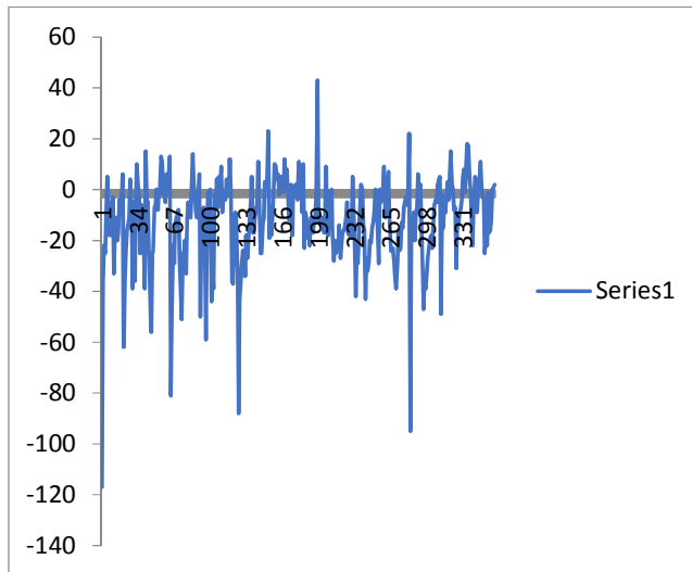
Figure 1: Graphical representation of 2015 and 2016, Disturbance Storm Time
