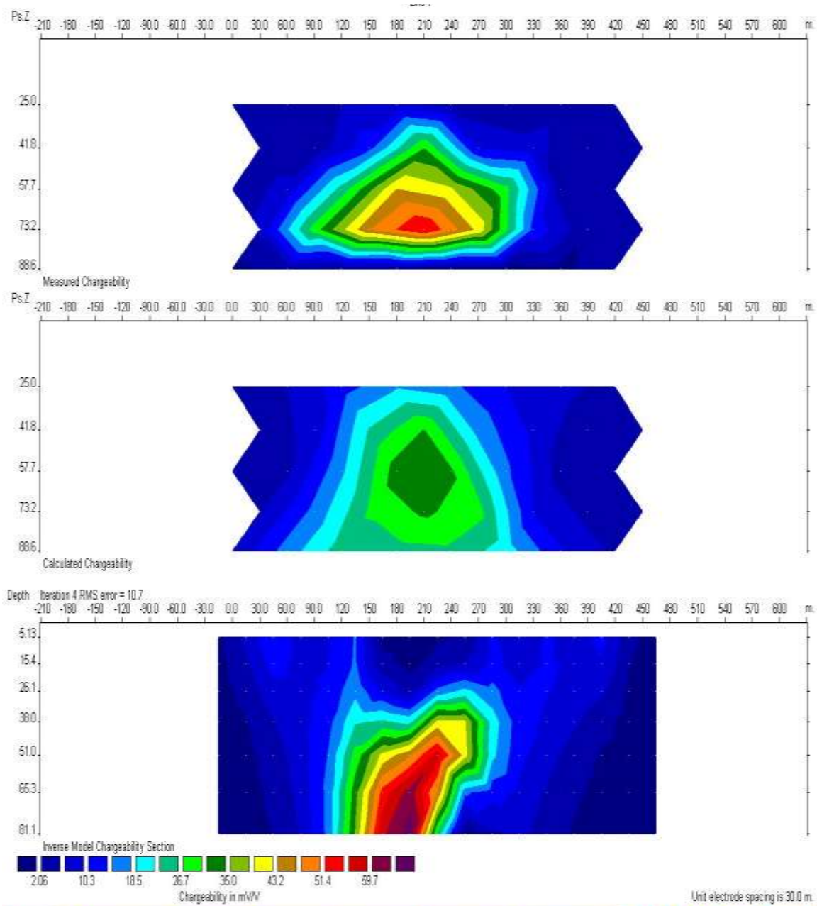
Fig.9: Pseudosection for measured chargeability, calculated chargeability and inverse model chargeability section for line 1.
