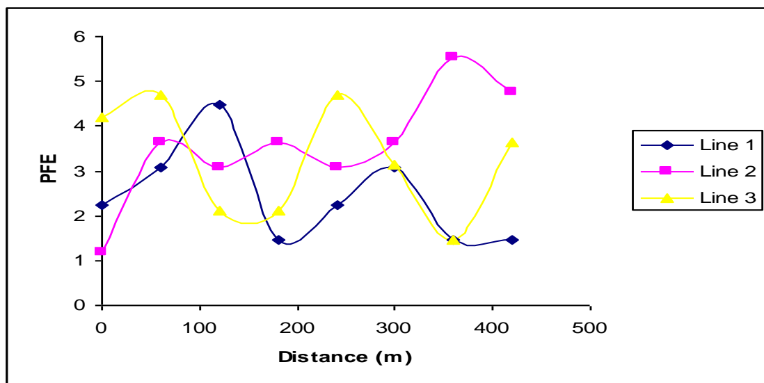
Fig. 5: Plot of Percentage frequency effect at 3Hz for the lines
