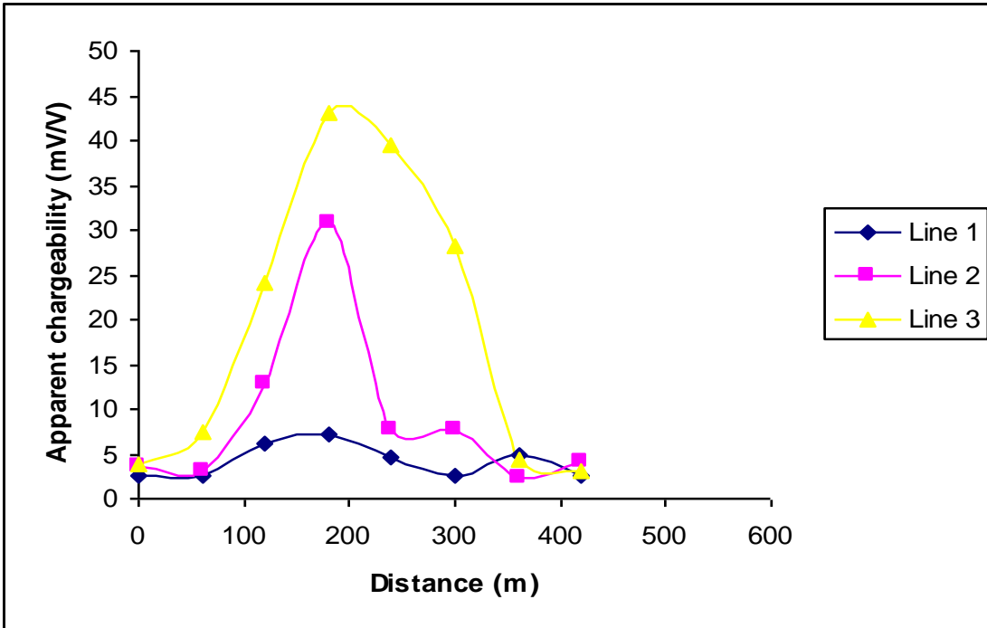
Fig .7: Plot of Apparent chargeability vs distance for the lines
