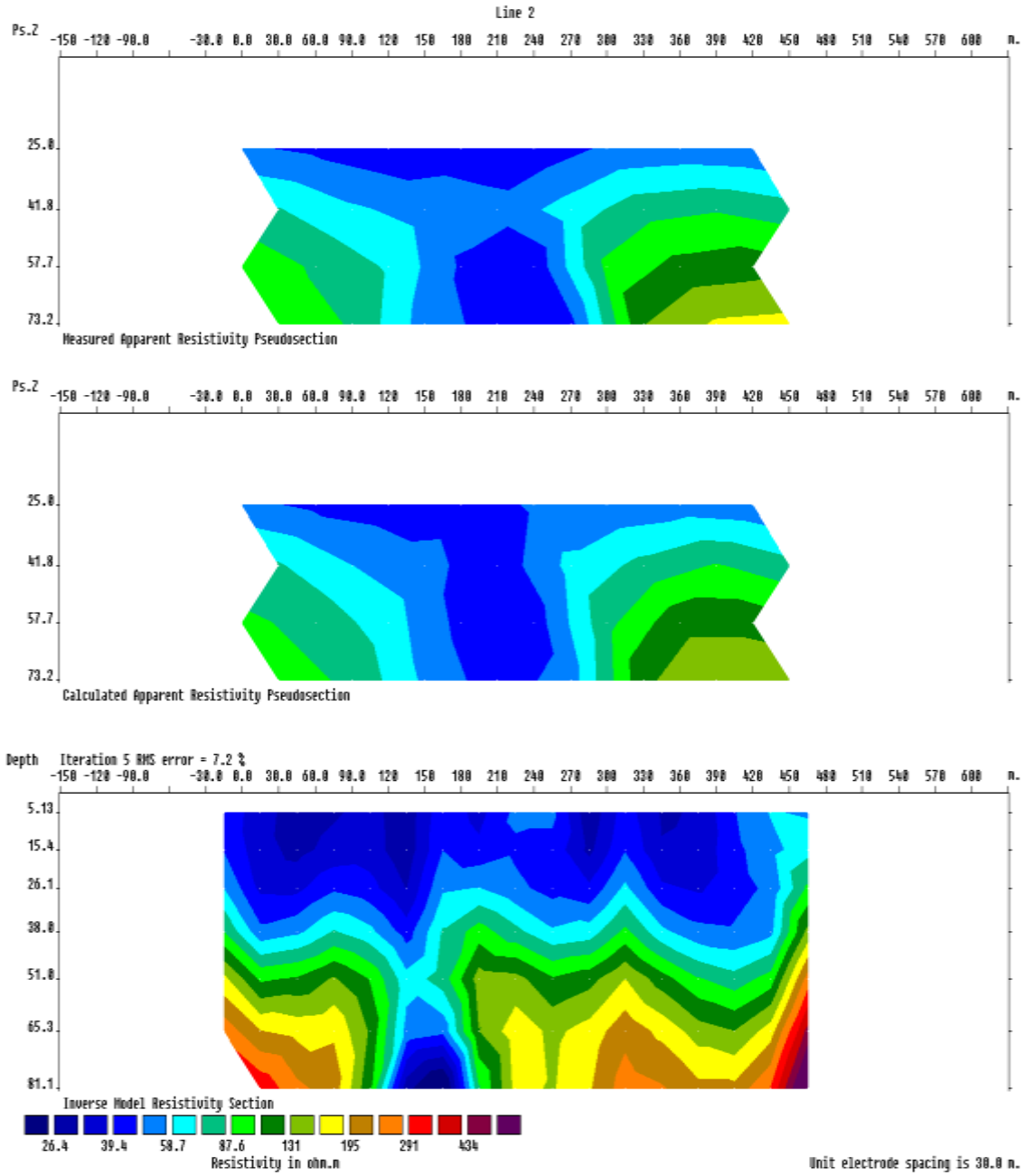
Fig.10: Pseudosection for measured, calculated and inverse model resistivity section for line 2
