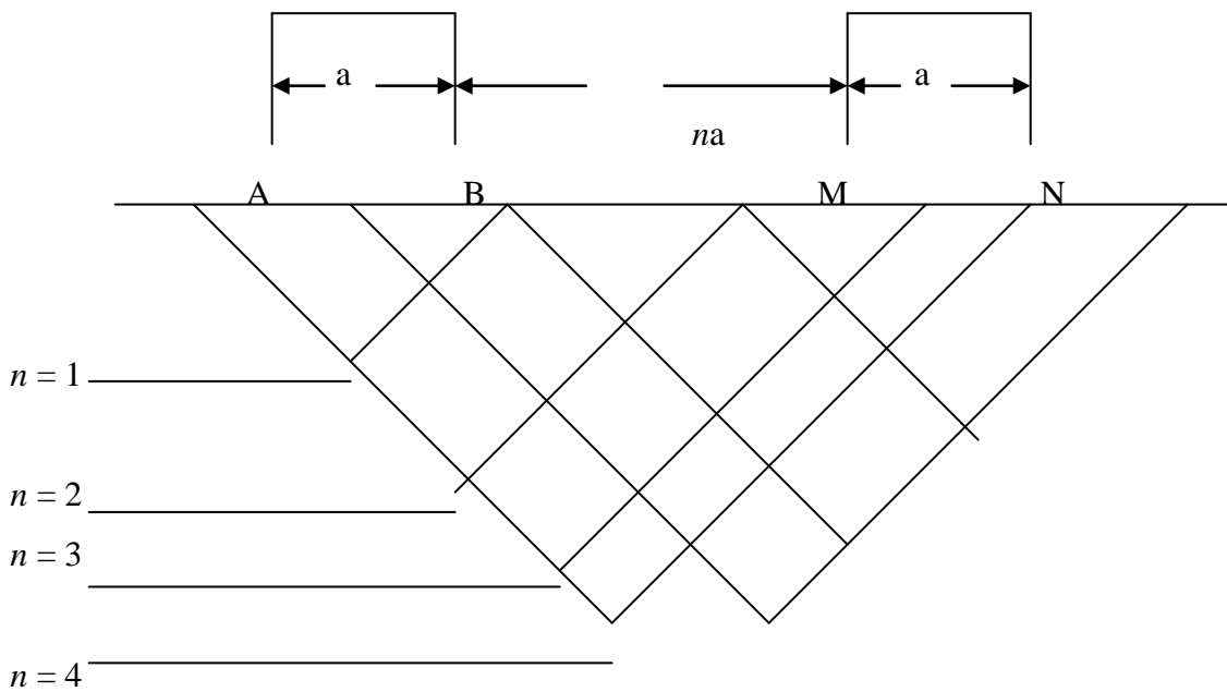
Fig.3: Convectional dipole-dipole pseudo-section plot.
