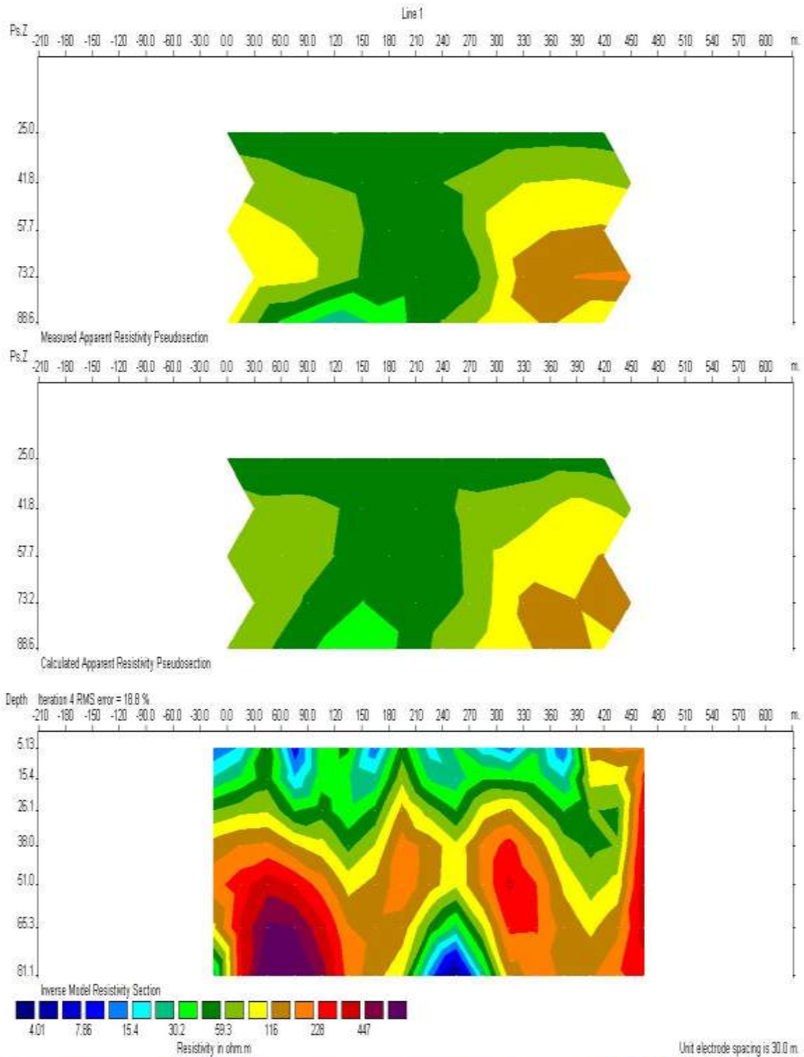
Fig.8: Pseudosection for measured, calculated and inverse model apparent resistivity for line 1.
