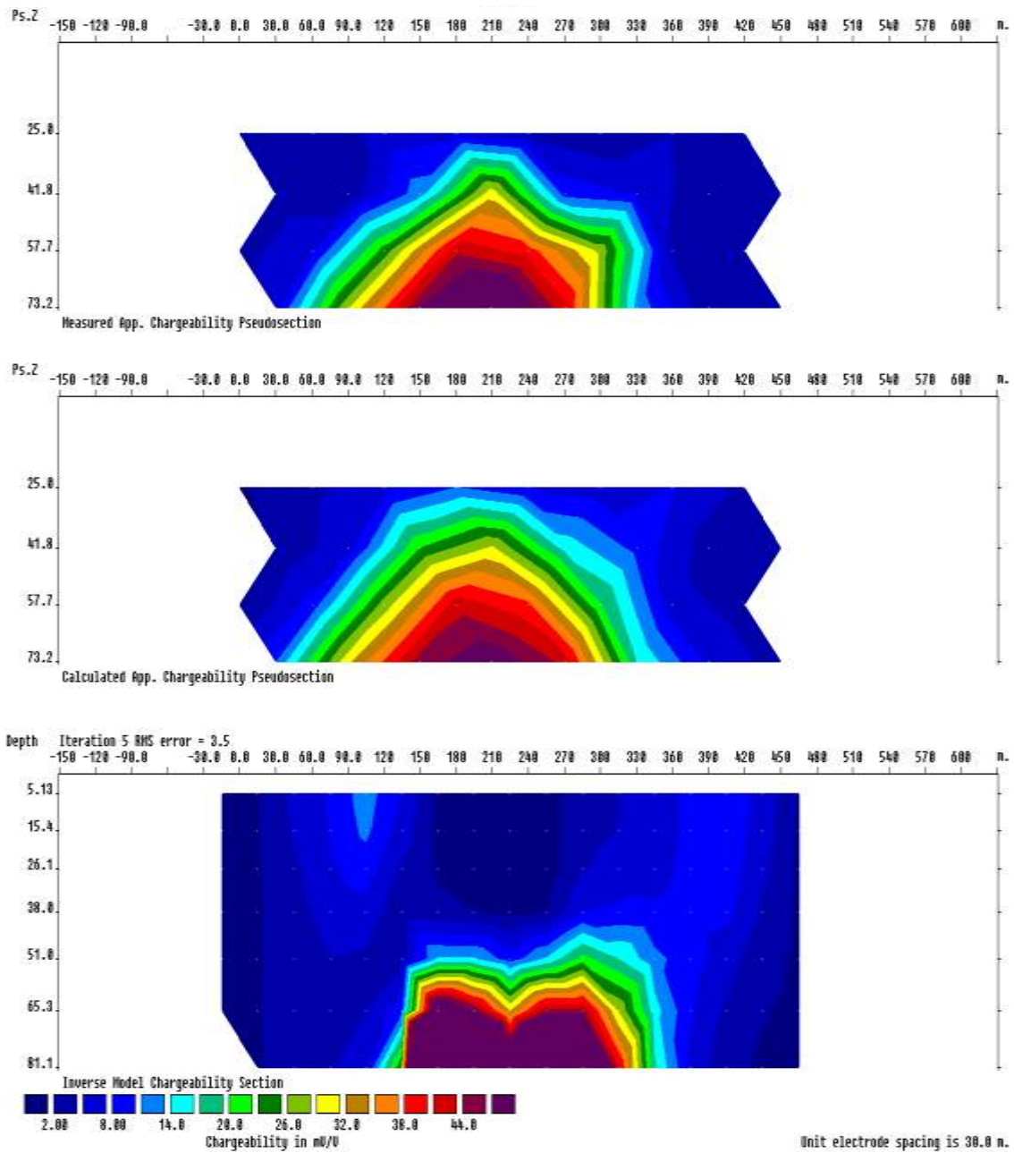
Fig. 11: Pseudosection for measured, calculated, and inverse model chargeability for line 2
