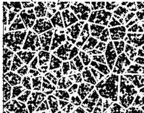
Fig. 7(b): Annealed 0.33% carbon (Model)
