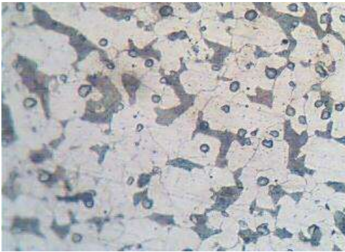
Fig.4(a): Annealed 0.23% carbon (Micrograph) X200
