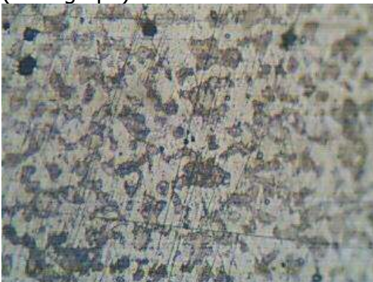
Fig. 7(a): Annealed 0.33% carbon (Micrograph) X200
