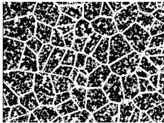
Fig.8(b): Annealed 0.47% carbon (Model)
