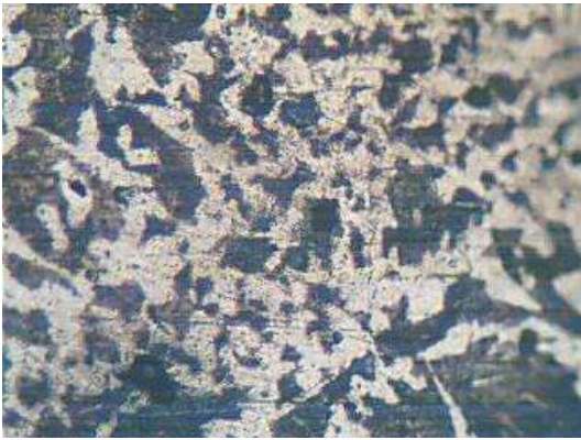
Fig.8(a): Annealed 0.47% carbon (Micrograph)X200
