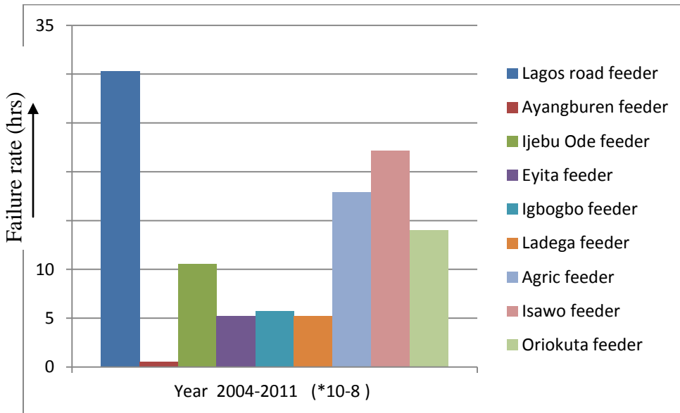
Figure 4.5. Reliability of the 11 kV Feeders (Year 2004–2011)
