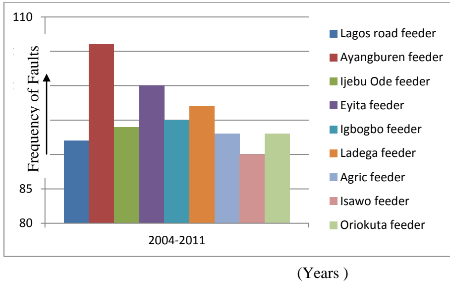
Figure 4.3: Frequency of Faults on 11 kV Feeders (Frequency of Faults on the three Phases) (2004–2011)
