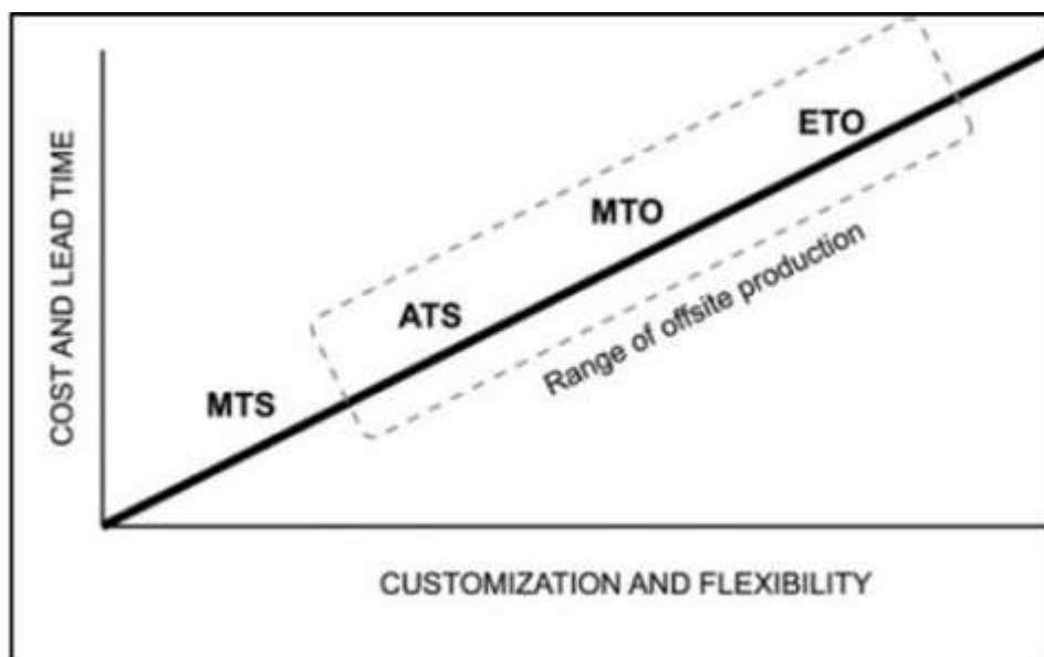
Figure 9: Range of Off-site Production in the Construction Sector Source: Graph courtesy of R.E. Smith
